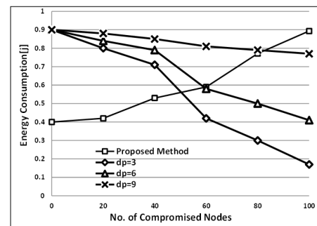
Figure 8. The network energy consumption vs. number of compromised nodes.
