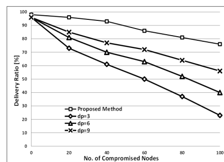
Figure 9. Packet delivery ratio vs. number of compromised nodes.
